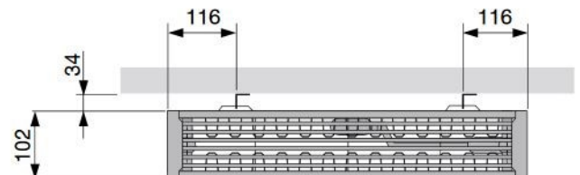
T22 | Top view
