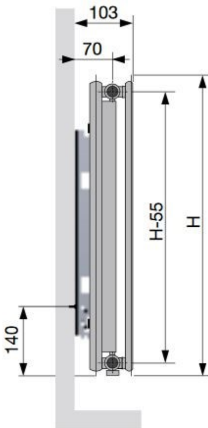
T21S | Side view
