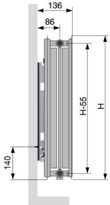
T22 | Side view
