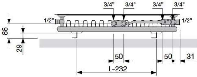
T21S | Bottom view
