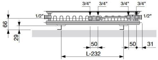
T22 | Bottom view
