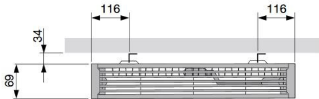
T21S | Top view
