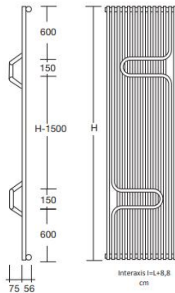
STANDARD HYDRAULIC VERSION WITH DOUBLE HANDLE (Connectors OC1)
