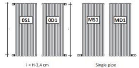
STANDARD HYDRAULIC VERSION WITH DOUBLE HANDLE (Connectors OC1)
