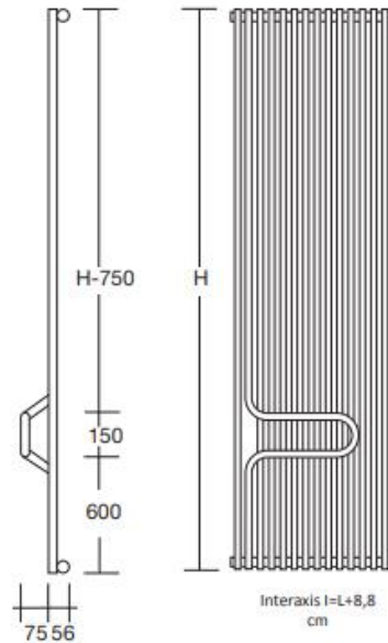
STANDARD HYDRAULIC VERSION (Connectors OC1)
